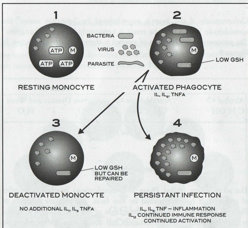
Figure 6—Immunologic activation by foreign substances causes production of inflammatory cytokines and expends GSH and energy. If invaders killed, system becomes quiet. If invader persists, continued expenditure of GSH and energy (ATP) and persistent inflammation.
